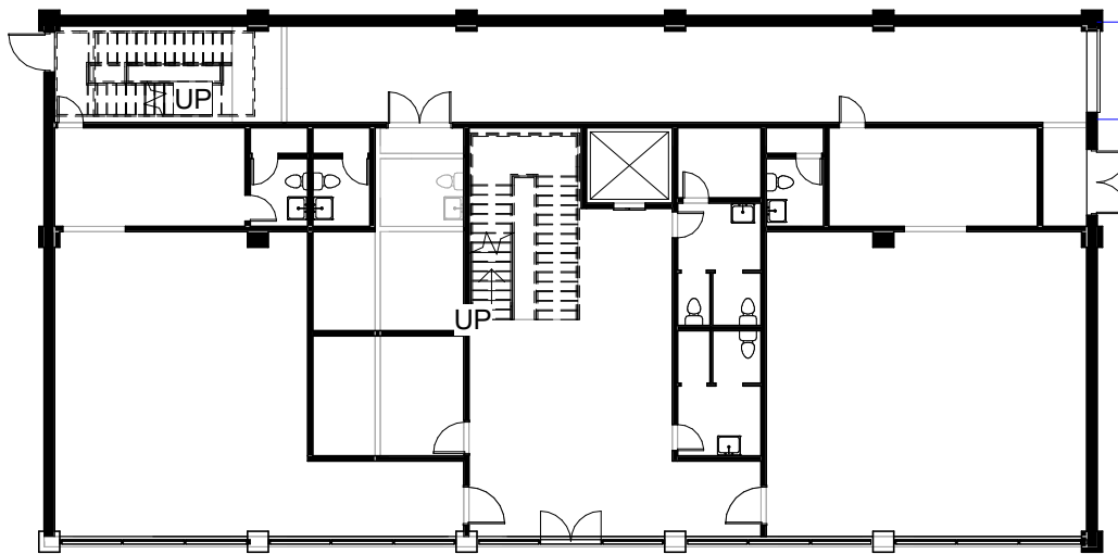
② Level 2 1" = 20'-0"
