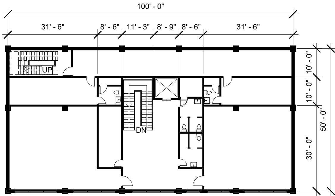
② Level 2 1" = 20'-0"
